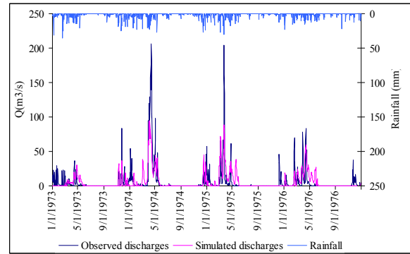
Figure 2. Sequential plot of the daily observed and modeled discharges and the rainfall at Ndgalu for the calibration period 1973-1976
