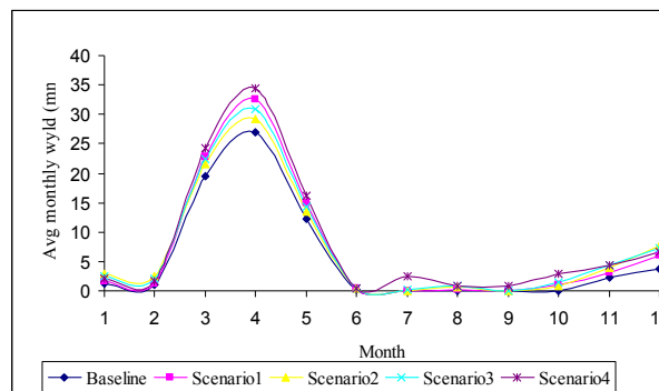
Figure 6. Change in average monthly stream flows predicted for scenarios 1 - 4 relative to the baseline over the 4 year simulation period
