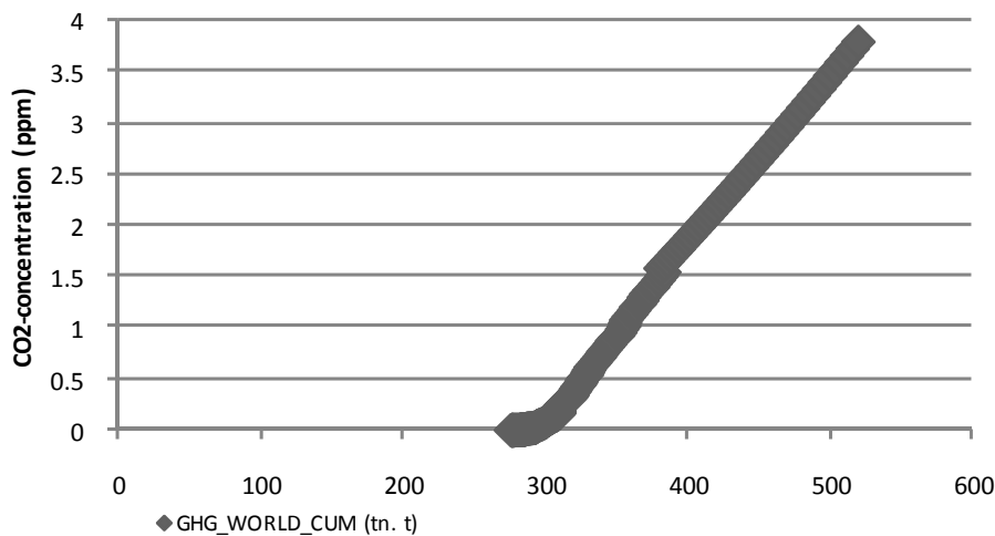
Figure 2. Cumulated GHG-emissions and CO 2 -concentration (ppm). Source: [12].
