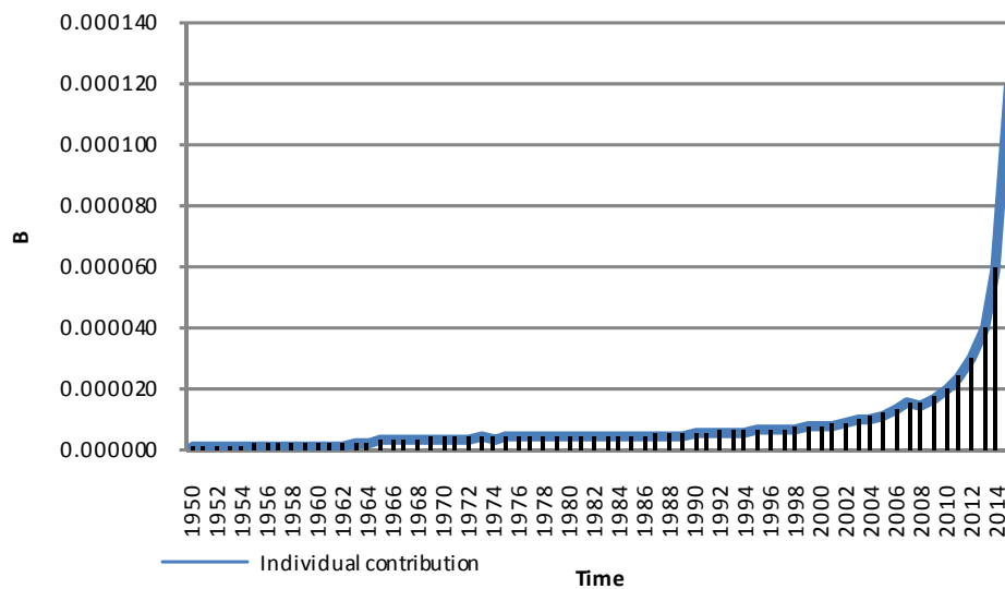
Figure 1. Development of individual contribution to climate change (ex post, 1950-2030). Source: [12], own calculation.
