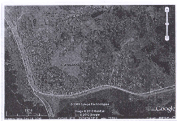
Figure 3: View of Uwanjani gully and built-up areas threatened by gully extension
